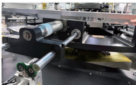
▲ Printing jig
