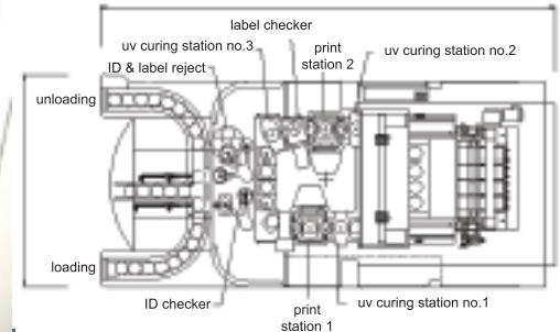
Layout of HS-480WD
