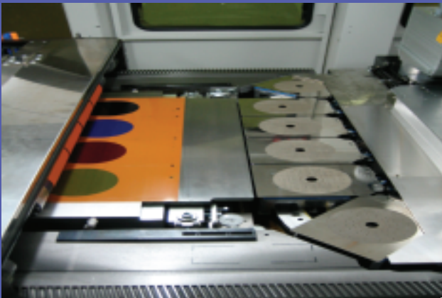
Printing Conveyor with vacuum plate holder
