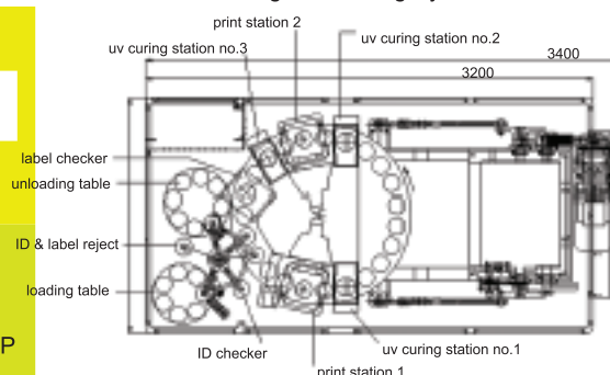
Loading / Unloading System
