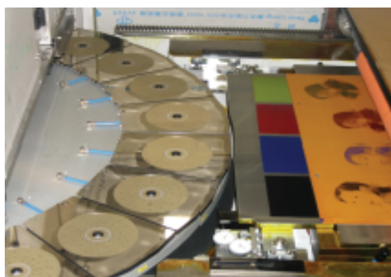
Printing Table with vacuum plate holder
