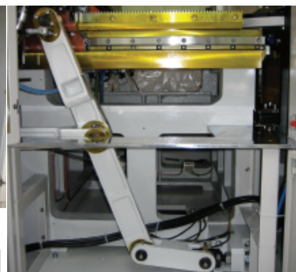
Two offset head supporting arm in both sides
